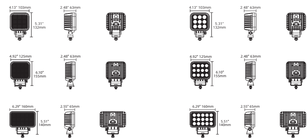
PART NO. 4C-ZB-Y
